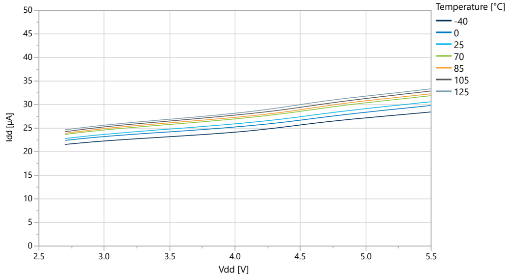
Figure 33-31. BOD Current vs. V_{DD} (Continuous Mode Enabled)
