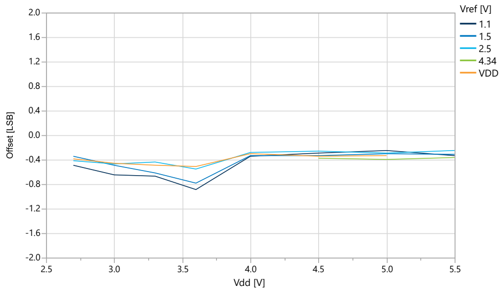
Figure 33-44. Offset Error vs. V_{DD} ( f_{ADC}=115 kps) at T=25^{\circ}C , REFSEL = Internal Reference
