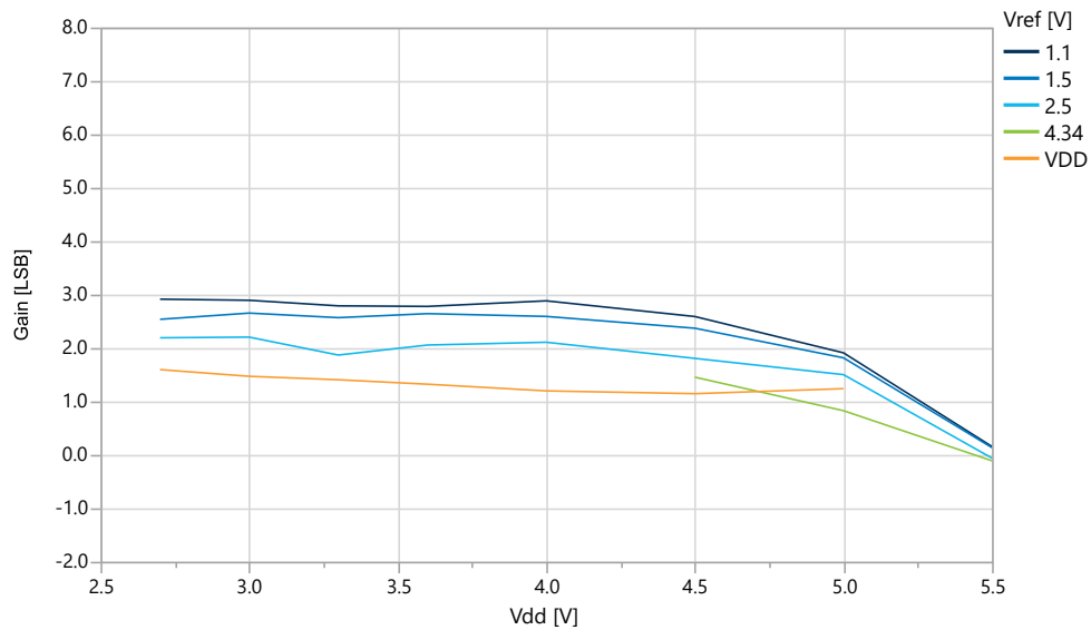
Figure 33-40. Gain Error vs. V_{DD} ( f_{ADC}=115 ksp/s) at T=25^{\circ}C , REFSEL = Internal Reference
