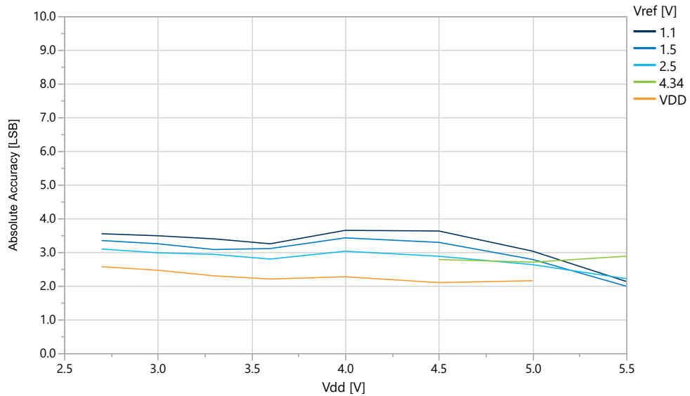
Figure 33-36. Absolute Accuracy vs. V_{DD} ( f_{ADC}=115 kps) at T=25^{\circ}\text{C} , REFSEL = Internal Reference
