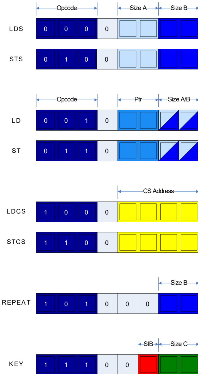
Figure 31-8. UPDI Instruction Set Overview
