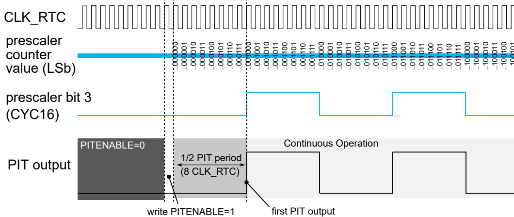
Figure 23-2. Timing Between PIT Enable and First Interrupt Enabling PIT with RTC/Prescaler Disabled
