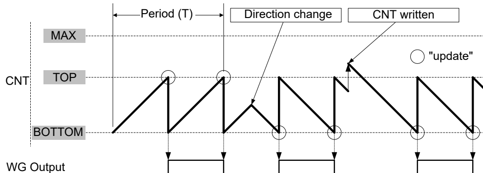
Figure 21-9. Frequency Waveform Generation
