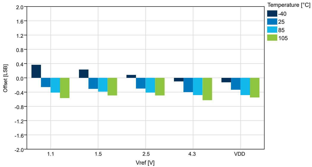
Figure 33-45. Offset Error vs. V_{ref} ( V_{DD}=5.0V , f_{ADC}=115 kps), REFSEL = Internal Reference
