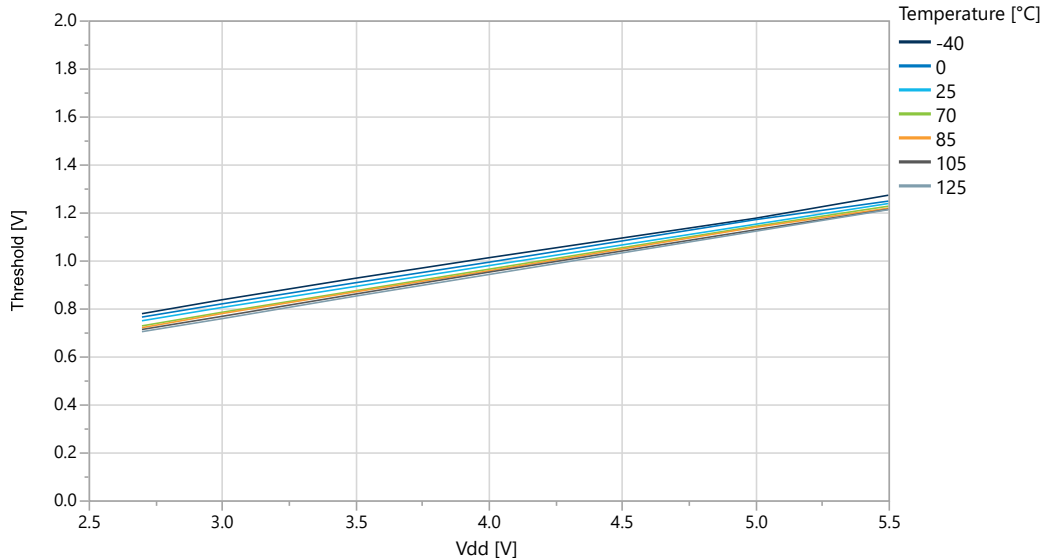
Figure 33-15. I/O Pin Input Hysteresis vs. V_{DD}
