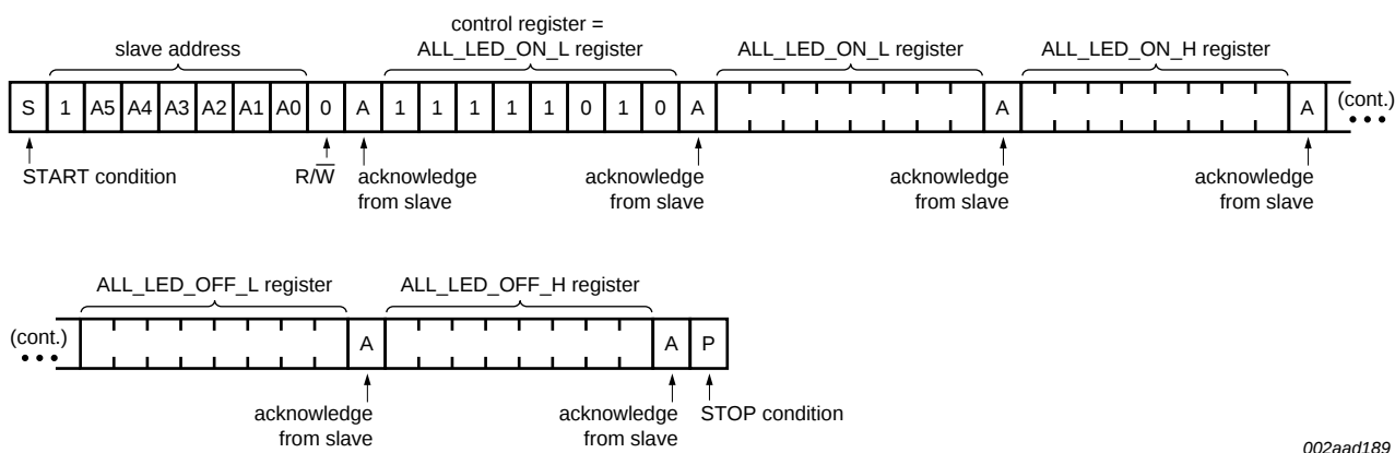
Fig 23. Write to ALL_LED_ON and ALL_LED_OFF registers using the Auto-Increment feature; AI initially set
