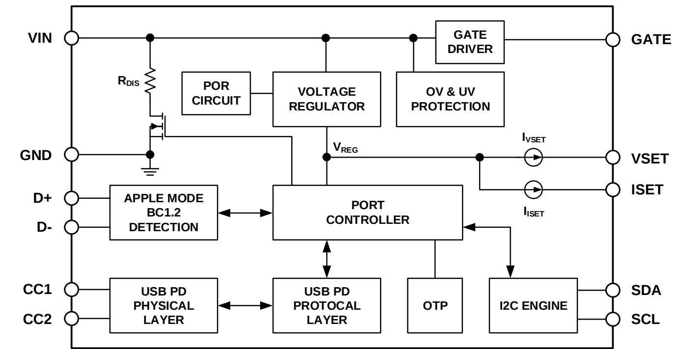
Figure 3. HUSB238 Functional Block Diagram
