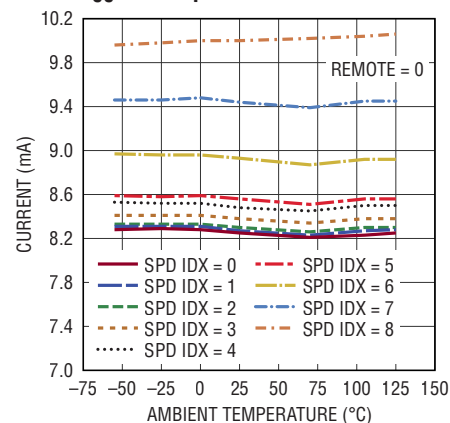
I_{CC} vs Temperature I 2 C Bus Idle
