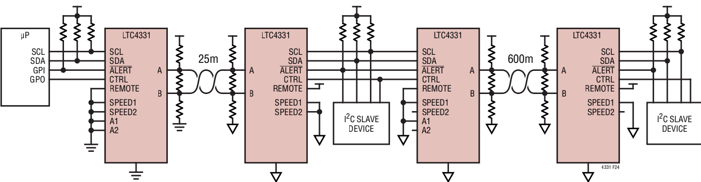
Figure 24. Multi-Tier Extender Network
